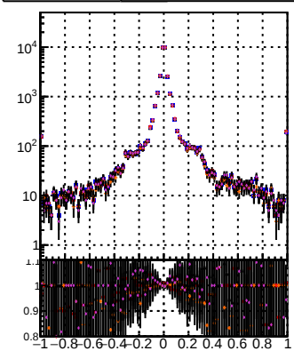
Orig/DOM orig MS N of reco track vs dxy(PV) N of associated (recoToSim) tracks vs dxy(PV) N of associated (recoToSim) loop tracks vs dxy(PV) detached/DOM orig MS
