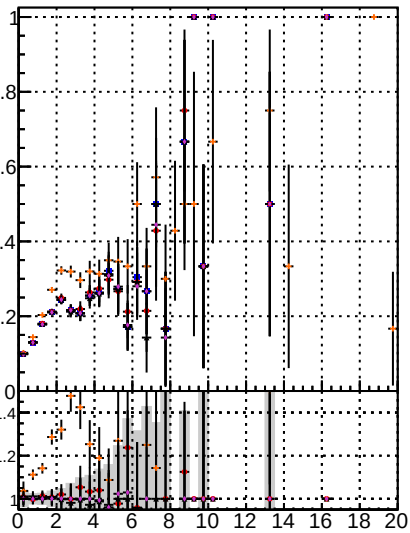
Fake rate vs. Orig/DQM_orig_MS MinibDQM_orig_MS MinibDQM_detached_orig_MS detached/DQM_orig_MS
