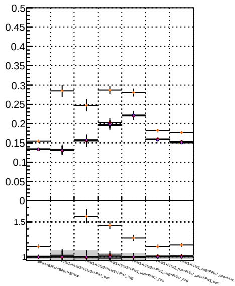
Fake rate vs. Orig/DQM_orig_MS MinibDQM_orig_MS MinibDQM_detached_orig_MS detached/DQM_orig_MS
