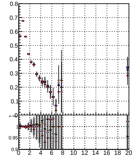
Fake rate vs. Orig/DQM_orig_MS Minibias/DQM_orig_MS detached/DQM_orig_MS
