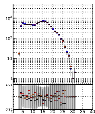
Orig/DQM orig MS duplicated/DQM orig MS hit/DQM orig MS detached/DQM orig MS
