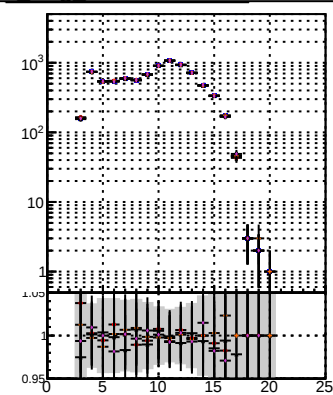
Orig/DQM orig MS duplicated/DQM orig MS hit/DQM orig MS detached/DQM orig MS
