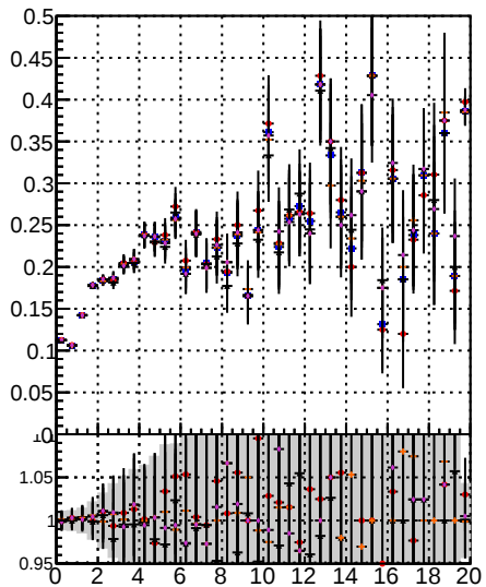
Fake rate vs. Orig/DQM_orig_MS Detached/DQM_orig_MS Orig/DQM_orig_MS Detached/DQM_orig_MS
