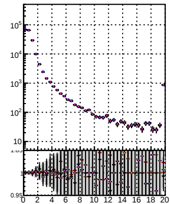
N of reco track vs. \chi^2 for different selection criteria
