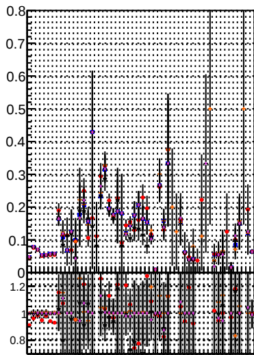
Fake rate vs. Orig/DQM_orig_MS Orig/DQM_orig_MS Detached/DQM_orig_MS Detached/DQM_orig_MS
