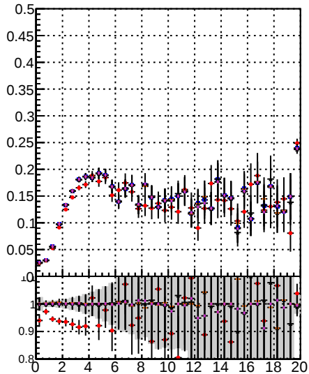
Fake rate vs. Orig/DQM_orig_MS Orig/DQM_orig_MS Detached/DQM_orig_MS Detached/DQM_orig_MS
