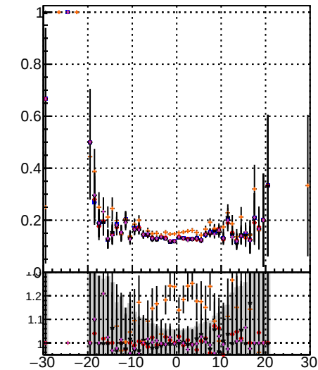
Orig/DQM_orig_MS higher/DQM_orig_MS detached/DQM_orig_MS Fake rate vs vertpos
