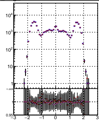
Orig/DQM_orig_MS recoToSim_orig_MS detached/DQM_orig_MS
