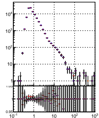
Orig/DQM_orig_MS recoToSim_orig_MS detached/DQM_orig_MS
