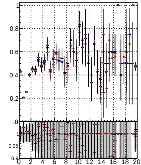
Fake rate vs. Orig/DQM_orig_MS Inner/DQM_orig_MS Detached/DQM_orig_MS
