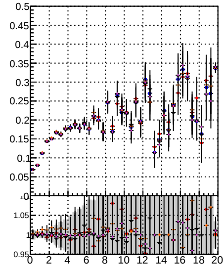
Fake rate vs. Orig/DQM, orig, MS detached/DQM, orig, MS
