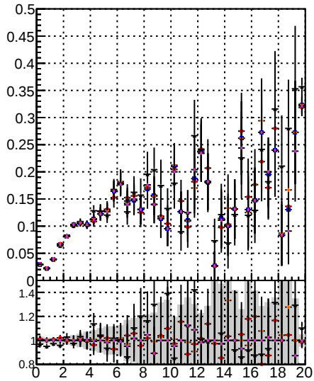
Fake rate vs. Orig/DQM_orig_MS Pileup/DQM_orig_MS Duplicates/DQM_orig_MS
