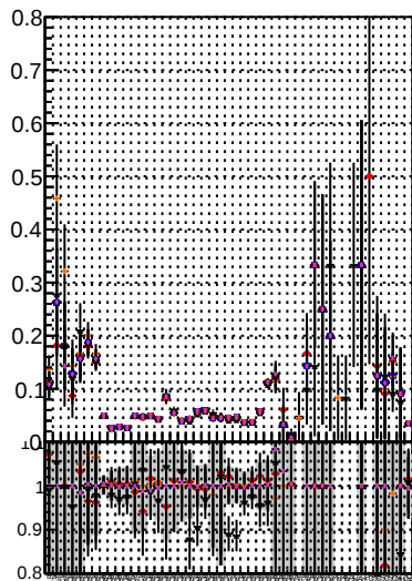
Fake rate vs. Orig/DQM_orig_MS Pileup/DQM_orig_MS Duplicates/DQM_orig_MS
