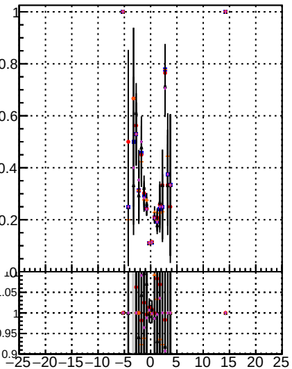
Fake rate vs d Orig/DQM_orig_MS Filtered/DQM_orig_MS Detached/DQM_orig_MS
