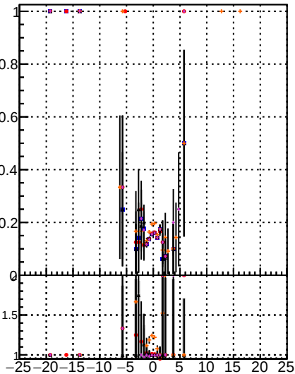
Orig/DQM_orig_MS DQM/DQM_orig_MS DQM/DQM_orig_MS detached/DQM_orig_MS
