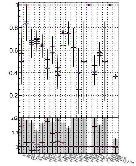
Fake rate vs. Orig/DQM orig MS Minus DQM orig MS Detached DQM orig MS
