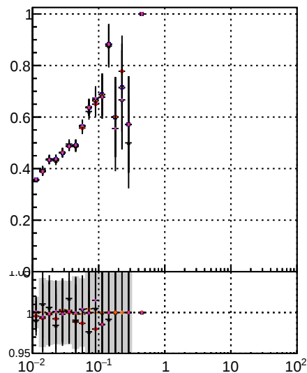
Fake rate vs v Orig/DQM_orig_MS higher ID Mer/DQM_orig_MS higher ID Mer/DQM_orig_MS detached V/DQM_orig_MS
