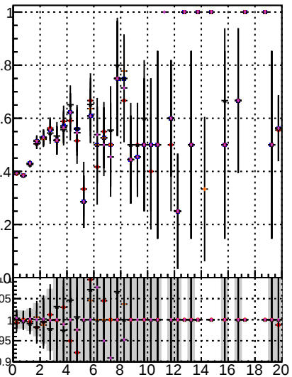
Fake rate vs. Orig/DQM_orig_MS MinibDQM_orig_MS Detached/DQM_orig_MS Detached/DQM_orig_MS
