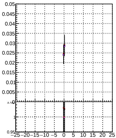
Fake rate vs d Orig/DQM_orig_MS MiniDQM_orig_MS detached/DQM_orig_MS
