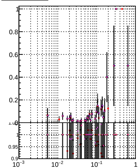
Fake rate vs \mu Orig/DQM_orig_MS higher/DQM_orig_MS detached/DQM_orig_MS
