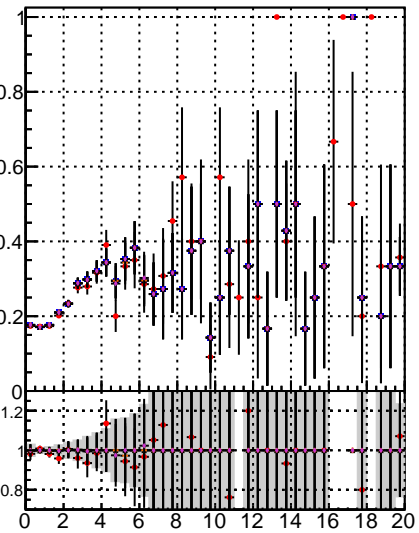
Fake rate vs. ◆ Orig/DQM_orig_MS ★ Attached/DQM_orig_MS ★ Detached/DQM_orig_MS
