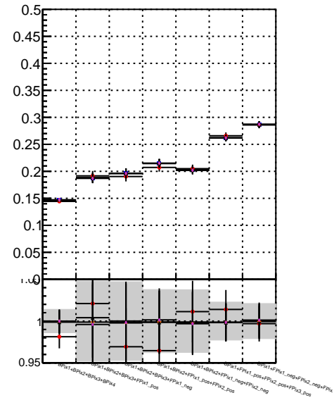
Fake rate vs. ◆ Orig/DQM_orig_MS ★ Attached/DQM_orig_MS ★ Detached/DQM_orig_MS
