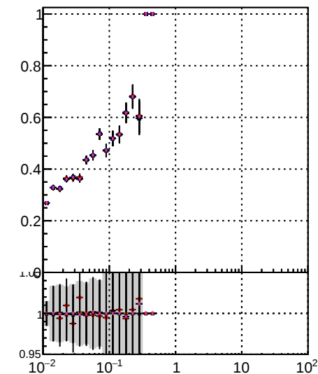
Fake rate vs v — Orig/DQM_orig_MS — higher ID/DQM_orig_MS — detached/DQM_orig_MS — detached w/DQM_orig_MS
