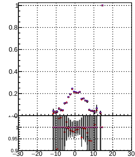
Fake rate vs v Orig/DQM_orig_MS higher ID/DQM_orig_MS higher ID/DQM_orig_MS detached V/DQM_orig_MS
