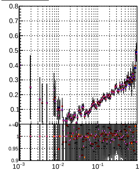
Fake rate vs \frac{\text{Orig/DQM\_orig\_MS}}{\text{higher/DQM\_orig\_MS}} \frac{\text{higher/DQM\_orig\_MS}}{\text{detached/DQM\_orig\_MS}}
