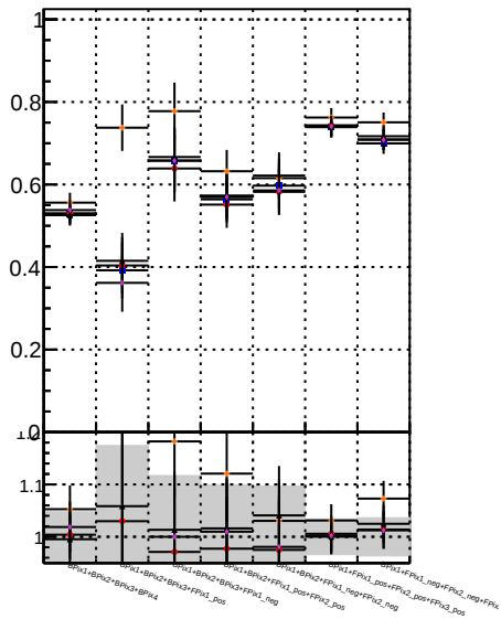
Fake rate vs. Orig/DQM_orig_MS Minibias/DQM_orig_MS Minibias/DQM_detached_MS detached/DQM_orig_MS
