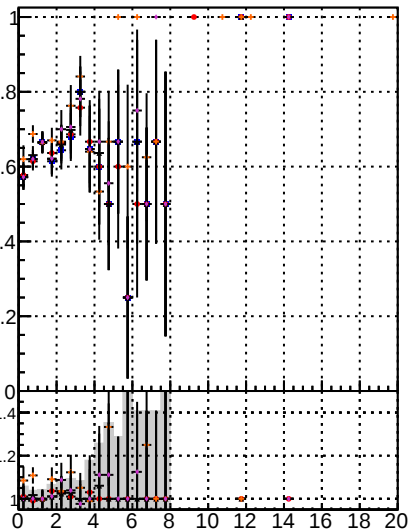
Fake rate vs. Orig/DQM_orig_MS Minibias/DQM_orig_MS Minibias/DQM_detached_MS detached/DQM_orig_MS
