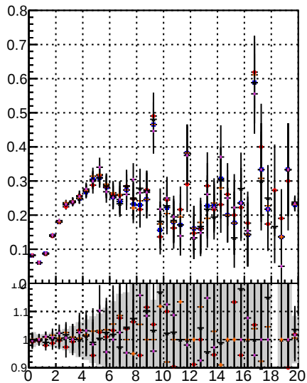
Fake rate vs. Orig/DQM_orig_MS Minus/DQM_orig_MS Minus/DQM_orig_MS detached/DQM_orig_MS
