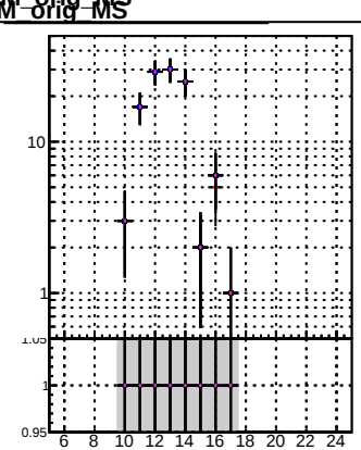
Orig/DQM orig MS hit/DQM orig MS hit/DQM orig MS detached/DQM orig MS
