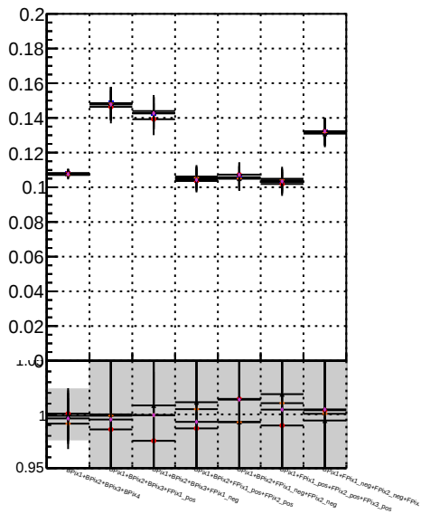
Fake rate vs. Orig/DQM_orig_MS Minibias/DQM_orig_MS Detached/DQM_orig_MS Minibias+Detached/DQM_orig_MS
