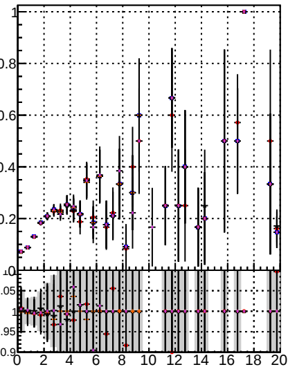
Fake rate vs. Orig/DQM_orig_MS Minibias/DQM_orig_MS Detached/DQM_orig_MS Minibias+Detached/DQM_orig_MS
