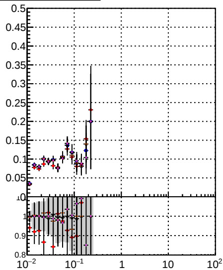
Fake rate vs v Orig/DQM_orig_MS higher ID Merger MS higher ID Merger DQM_orig_MS detached V/DQM_orig_MS
