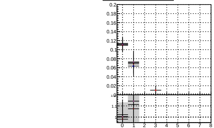
fake+duplicates vs pixel layers
