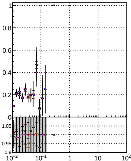
Fake rate vs v Orig/DQM_orig_MS higher ID/DQM_orig_MS higher ID/DQM_orig_MS detached/DQM_orig_MS
