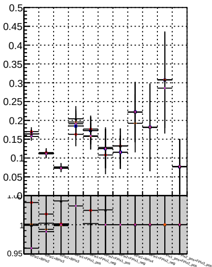
Fake rate vs. Orig/DQM orig MS MinibDQM orig MS MinibDQM orig MS detached/DQM orig MS
