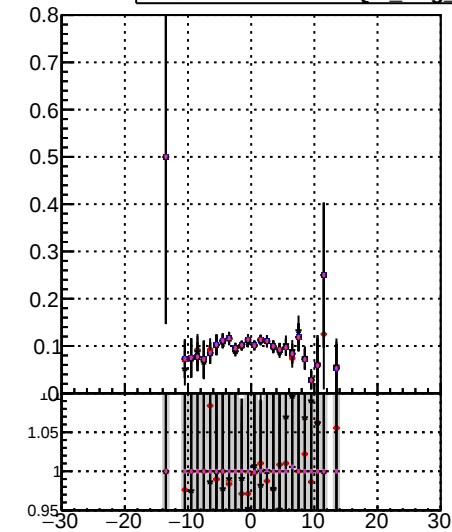
Fake rate vs vertpos Orig/DQM_orig_MS higherID/DQM_orig_MS detached/DQM_orig_MS
