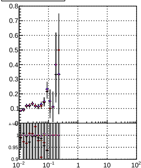
Fake rate vs vertpos Orig/DQM_orig_MS higherID/DQM_orig_MS detached/DQM_orig_MS
