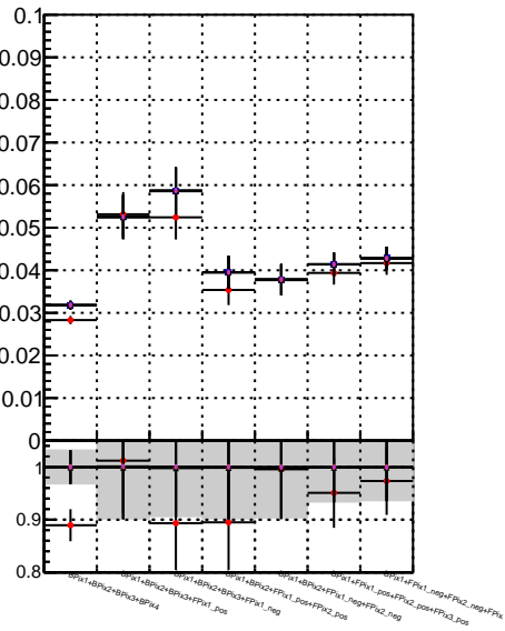
Fake rate vs. ● Orig/DQM_orig_MS ◆ Detached/DQM_orig_MS ▲ Detached/DQM_orig_MS ■ Detached/DQM_orig_MS
