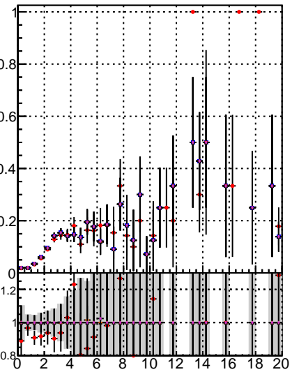
Fake rate vs. ● Orig/DQM_orig_MS ◆ Detached/DQM_orig_MS ▲ Detached/DQM_orig_MS ■ Detached/DQM_orig_MS
