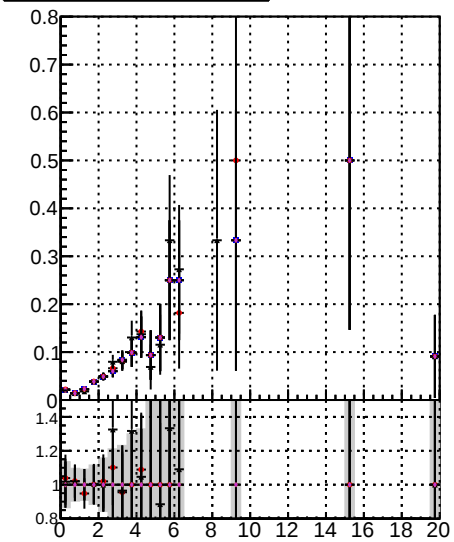
Fake rate vs. Orig/DQM_orig_MS Mixed/DQM_orig_MS detached/DQM_orig_MS
