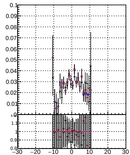
Fake rate vs d Orig/DQM_orig_MS MiniAOD/DQM_orig_MS detached/DQM_orig_MS
