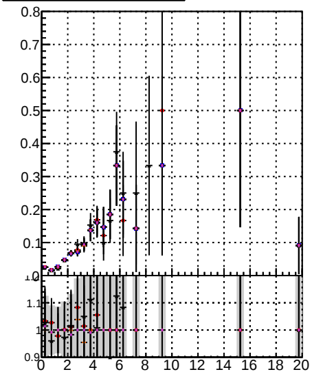
Fake rate vs. Orig/DQM_orig_MS Minus DQM_orig_MS detached/DQM_orig_MS
