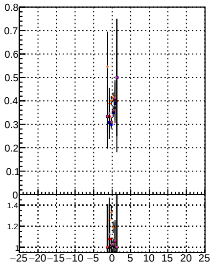
Fake rate vs d Orig/DQM_orig_MS Merged/DQM_orig_MS detached/DQM_orig_MS
