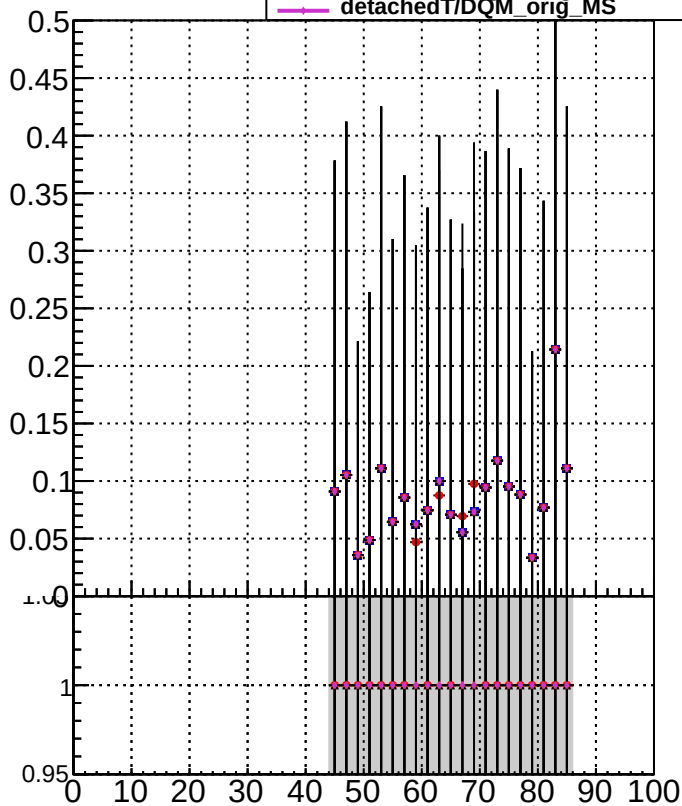
Orig/DQM_orig_MS initial/DQM_orig_MS highPtTriplet/DQM_orig_MS detachedQ/DQM_orig_MS detachedT/DQM_orig_MS
