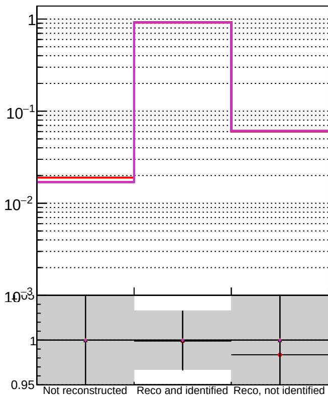
Orig/DQM_orig_MS initial/DQM_orig_MS highPtTriplet/DQM_orig_MS detachedQ/DQM_orig_MS detachedT/DQM_orig_MS
