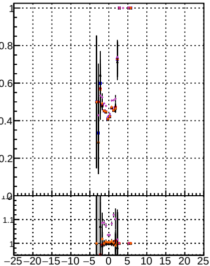
Fake rate vs d Orig/DQM_orig_MS Filtered/DQM_orig_MS detached/DQM_orig_MS
