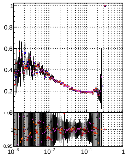
Pileup rate vs \frac{\text{Orig/DQM\_orig\_MS}}{\text{higher/DQM\_orig\_MS}}
