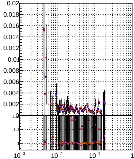
Duplicates Rate vs \frac{\text{Orig/DQM\_orig\_MS}}{\text{higher/DQM\_orig\_MS}}
