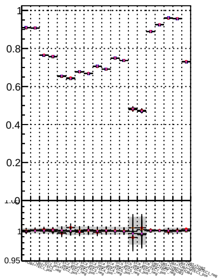
Fake rate vs. Orig/DQM orig MS DQM orig MS detached/DQM orig MS
