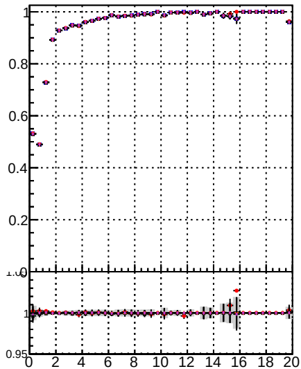
Fake rate vs. Orig/DQM orig MS DQM orig MS detached/DQM orig MS
