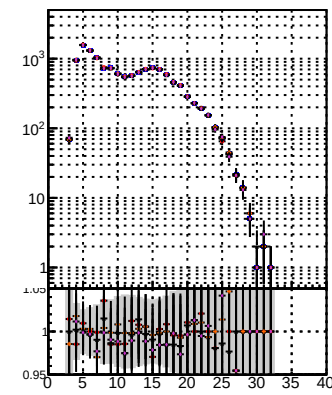
Orig/DOM orig MS dupl/DOM orig MS detached/DOM orig MS N of reco track vs hit
