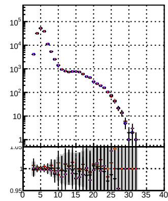
Orig/DOM orig MS dupl/DOM orig MS detached/DOM orig MS N of reco track vs hit
