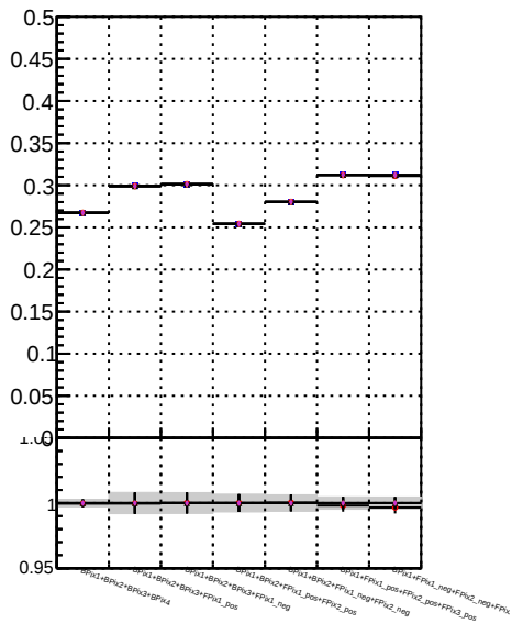
Fake rate vs. Orig/DQM_orig_MS Minibias/DQM_orig_MS detached/DQM_orig_MS
