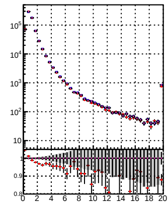
N of reco track vs. \chi^2 for Orig/DQM orig MS, detached/DQM orig MS, and detached/DQM orig MS
