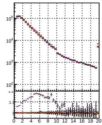
N of reco track vs. \chi^2 for different MS sets
