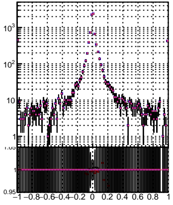
N of sim — Orig/DQM_orig_MS — initial/DQM_orig_MS — highPtTriplet/DQM_orig_MS — detachedQ/DQM_orig_MS — detachedT/DQM_orig_MS
