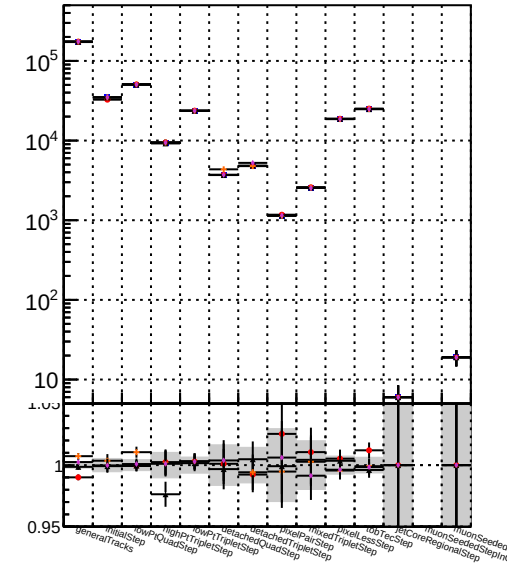
Number Color Label 1 Black high triplet/DOM_orig_MS 2 Orange detached O/DOM_orig_MS 3 Pink detached T/DOM_orig_MS
