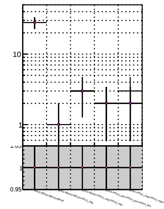
N of associated (recoToSim) loopier tracks vs normalized \chi^2 for different MS settings
