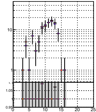
Orig/DQM orig MS high/DQM orig MS high/DQM orig MS detached/DQM orig MS
