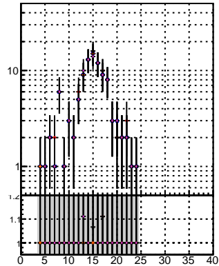
Orig/DQM orig MS high/DQM orig MS high/DQM orig MS detached/DQM orig MS
