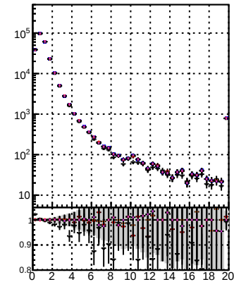
N of reco track vs. \chi^2 for different detector MS
